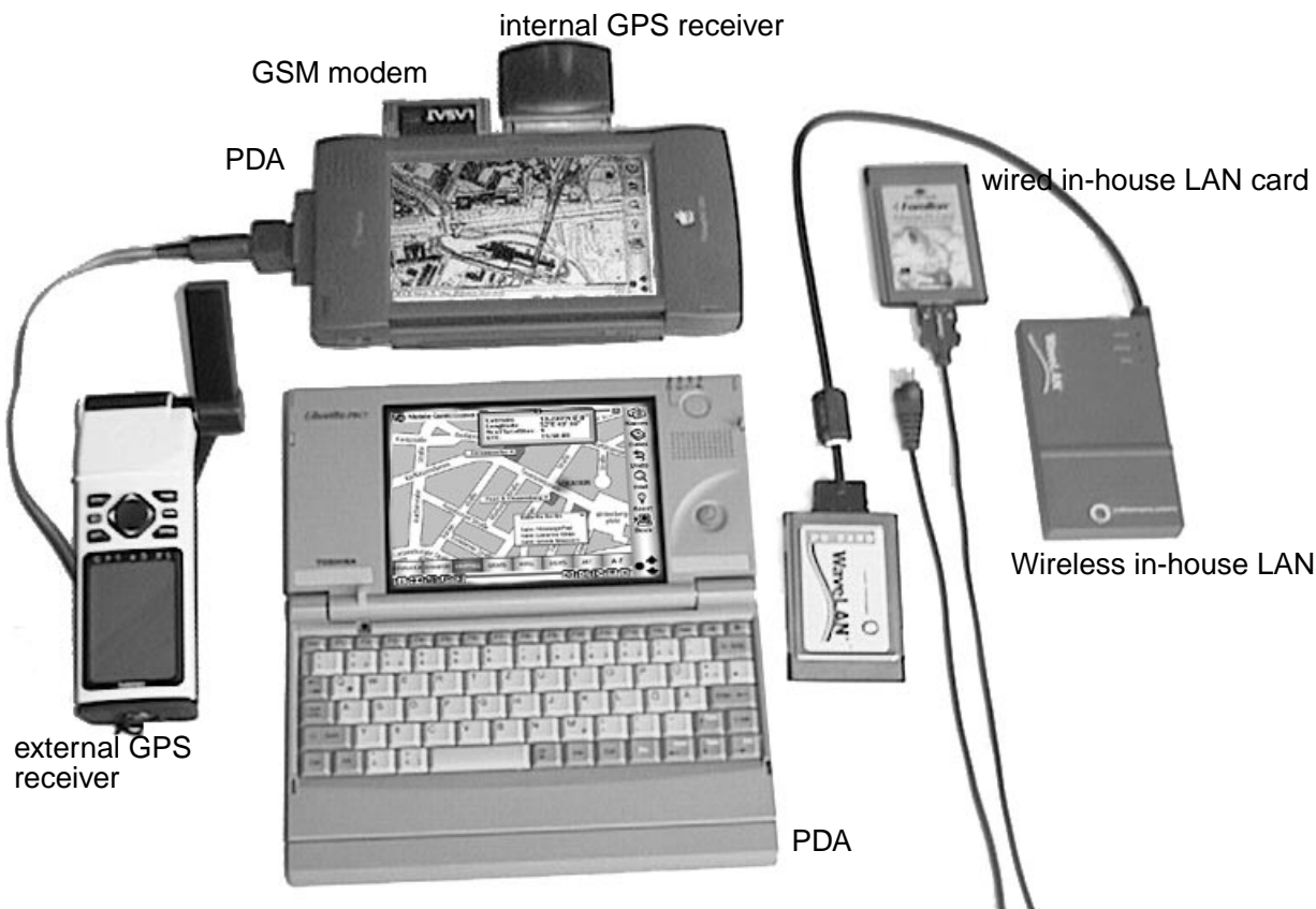
Figure 9 Compact PDA with integrated, exchangeable positioning and communication technology
