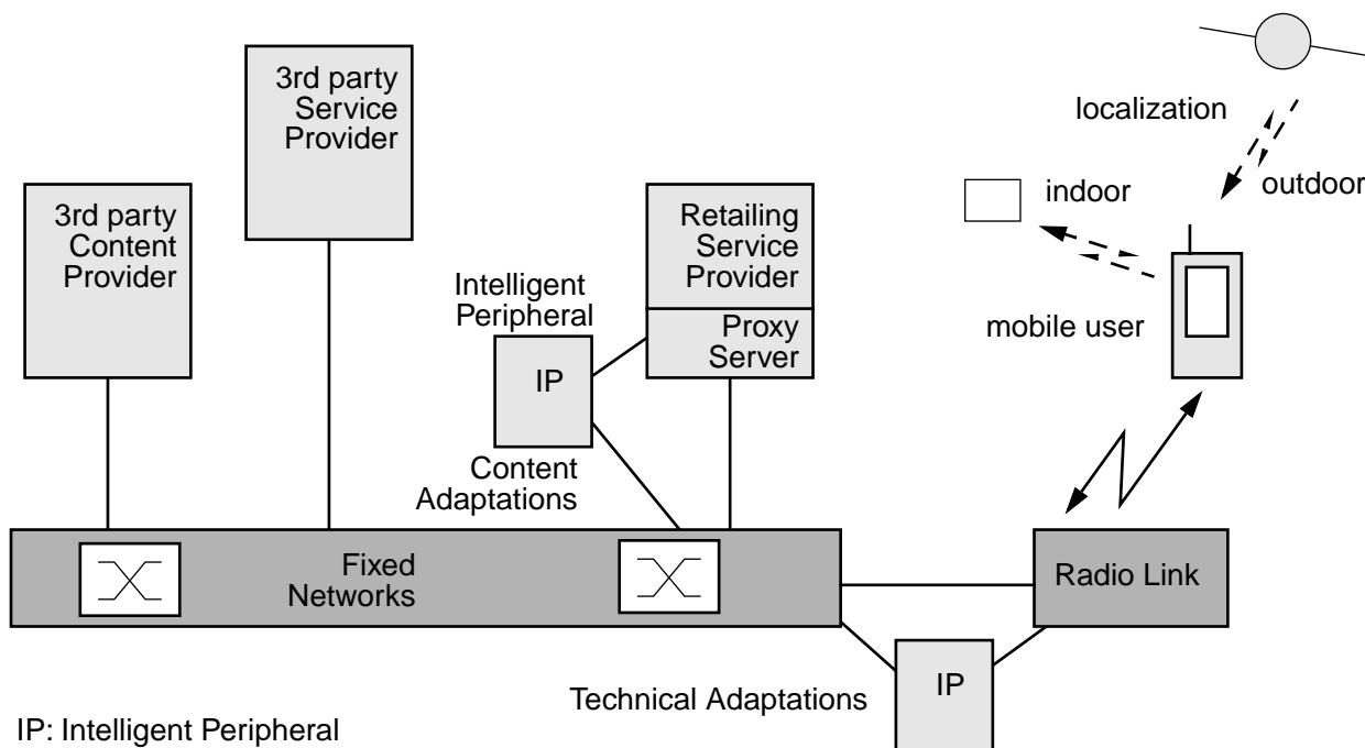
Figure 3 Technical System Architecture
