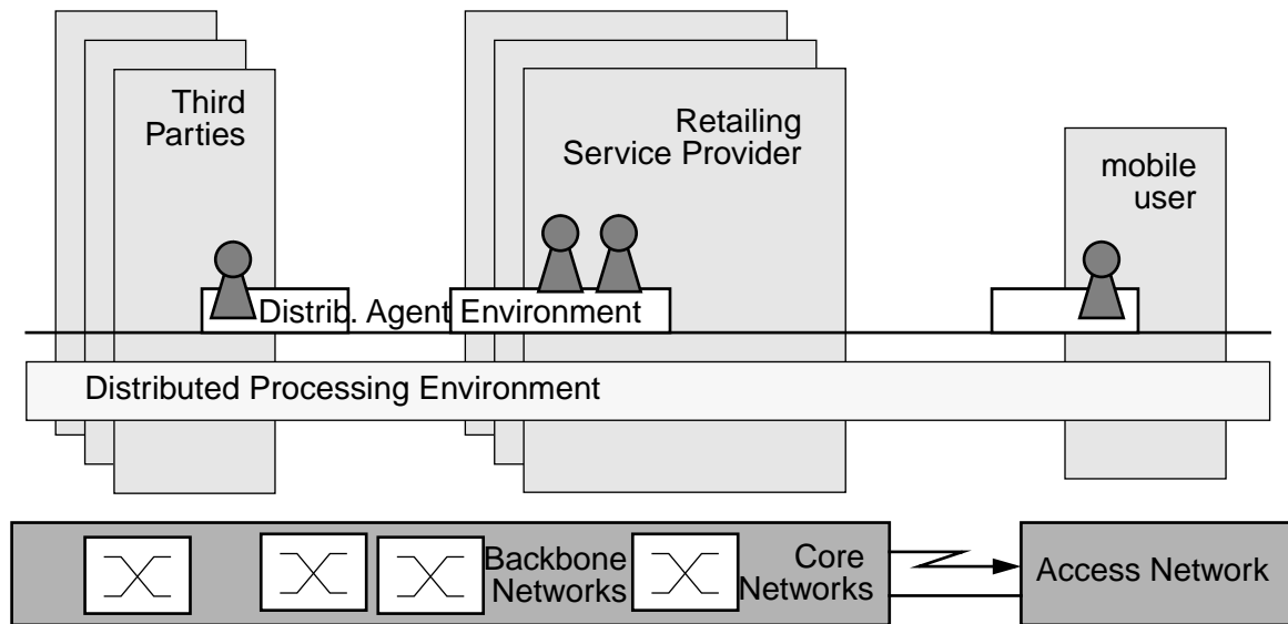
Figure 4 Middleware architecture for distributed processing and agent support
