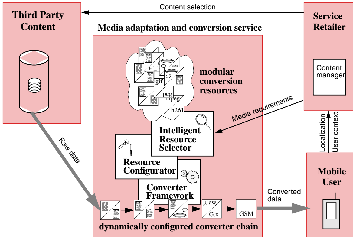
Figure 5 Dynamic Media Adaptation and Conversion Service
