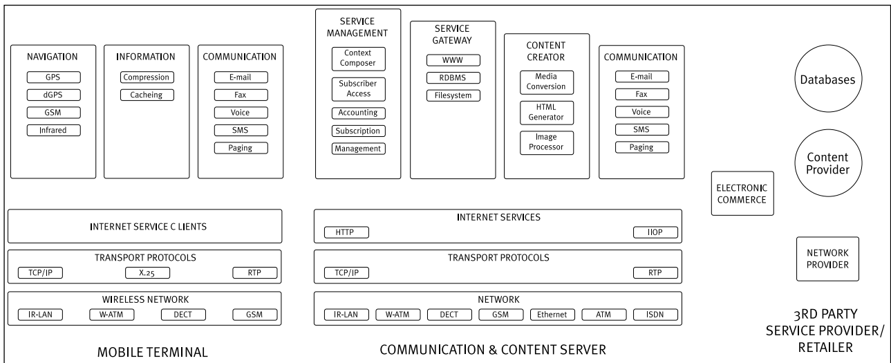
Figure 8 Mobile Guide system architecture
