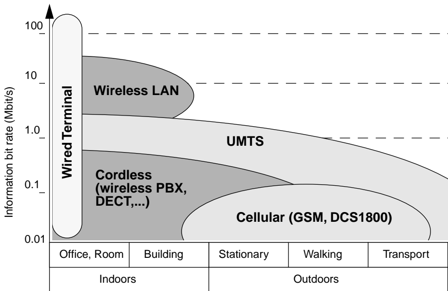
Figure 1 Comparison of Wireless Transmission Capabilities (after [1])
